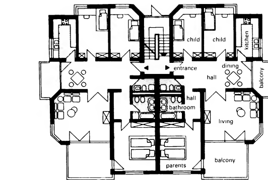
7 Two dwellings per floor
